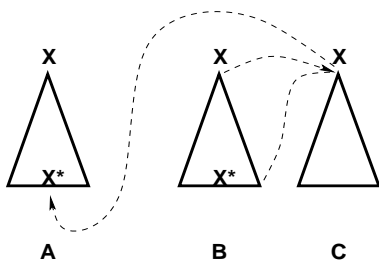
Figure 1: Flexible composition and adjoining at the same node. This is prohibited in TAG extensions without multiple adjoining.
